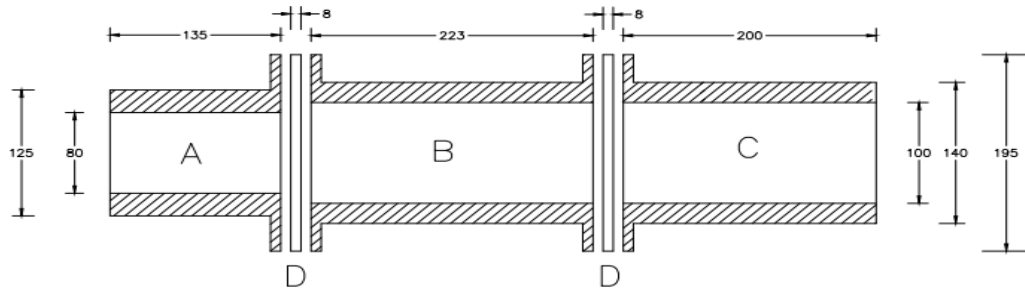
Figure Meta flex Coupling ( Dimensions)
